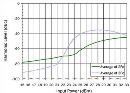
Harmonics (Temp. = 25 °C, V_{RF}(H) = 3 \text{ V} )
